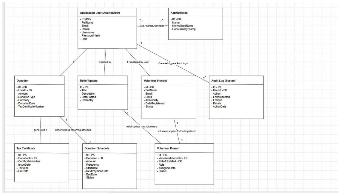
Figure X: Entity Relationship Diagram (ERD) for the Gift of the Givers Disaster Relief System.
