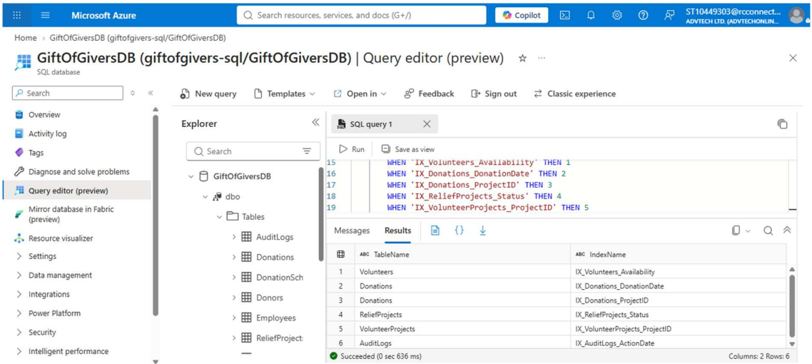
Figure X: Performance indexes implemented in the GiftOfGiversDB Azure SQL Database
